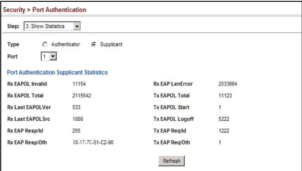
Figure 192: Showing Statistics for 802.1X Port Supplicant
