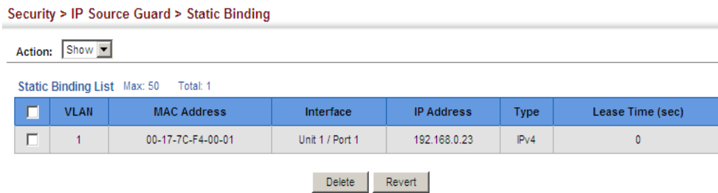
Figure 195: Displaying Static Bindings for IP Source Guard
