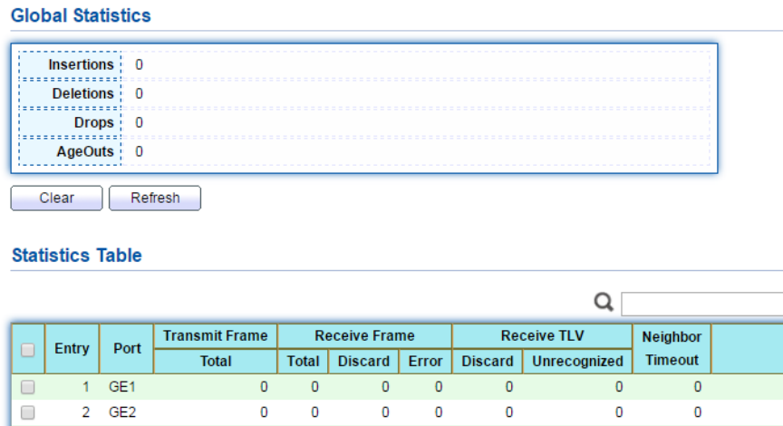
Figure 77 - Discovery > LLDP > Statistics
