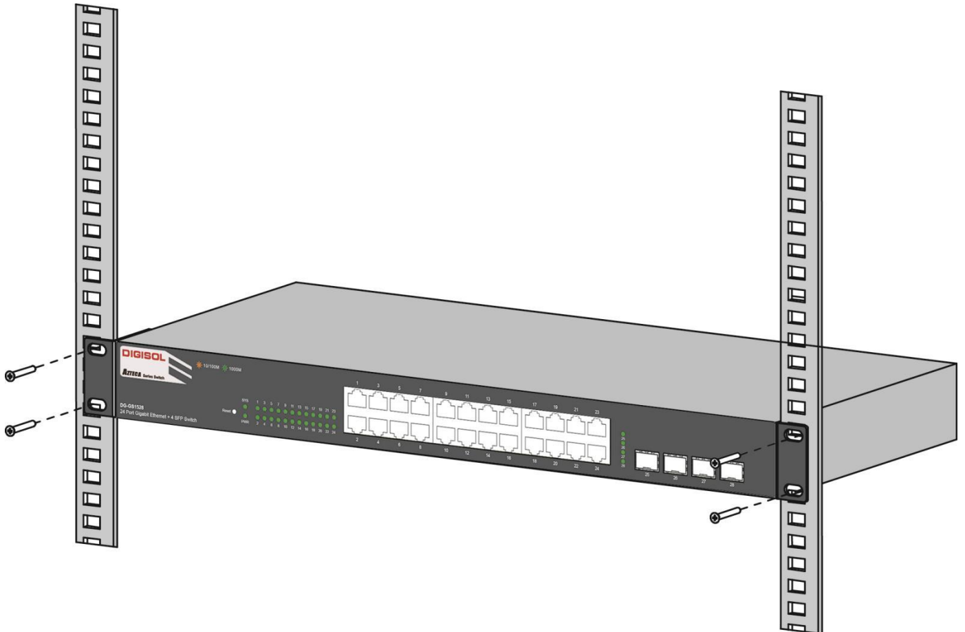
Figure 10 - Rack Installation
