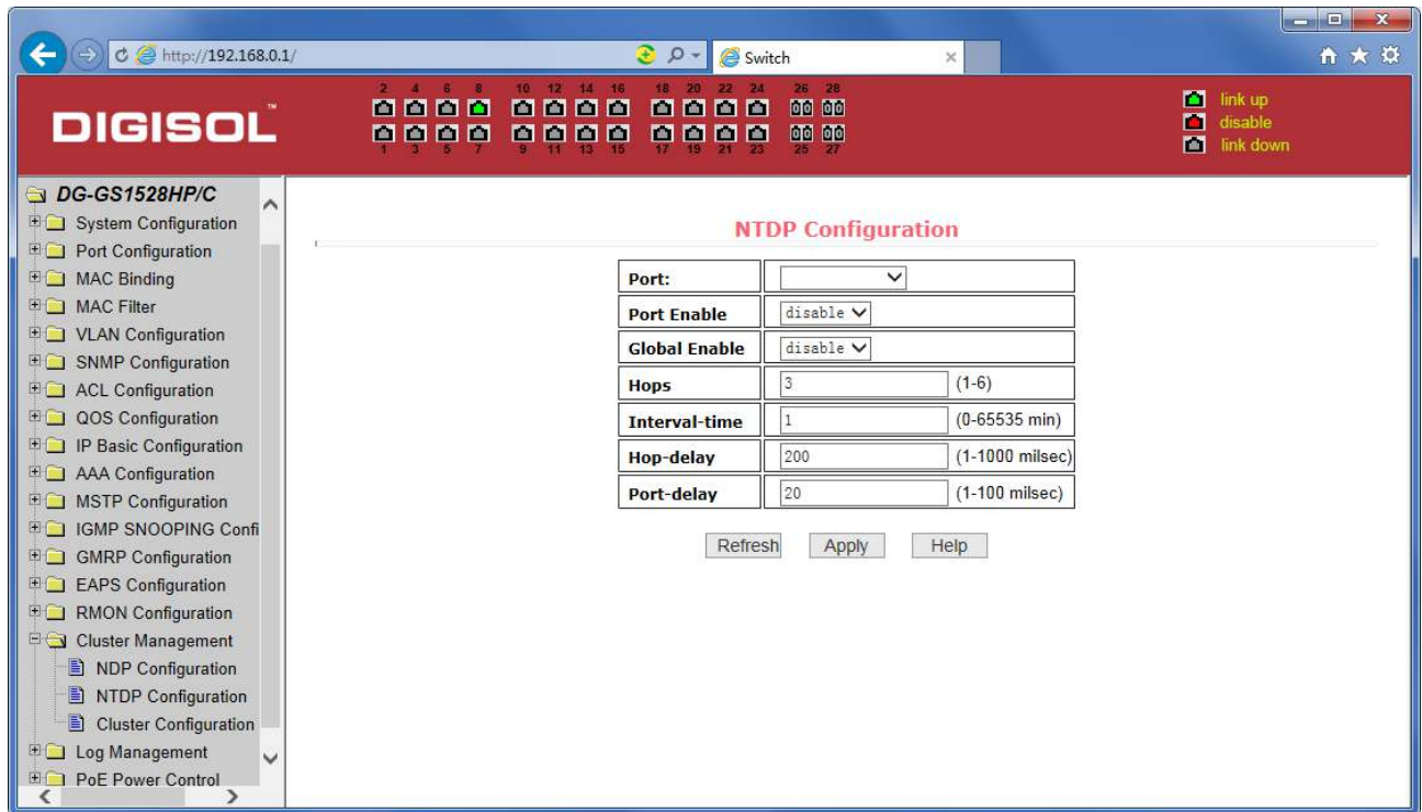
Figure 65 NTDP configuration page
