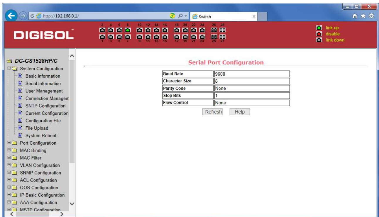
Figure 10 Serial port information page
