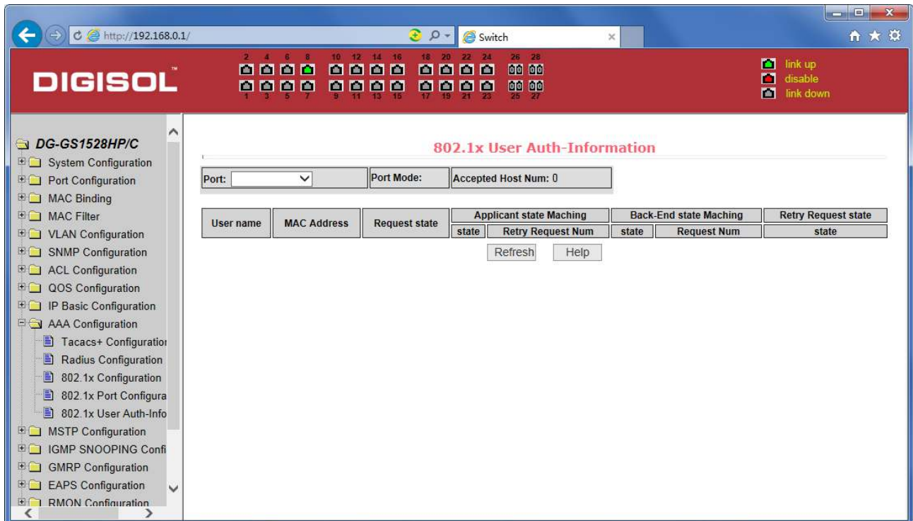
Figure 49 802.1x user authentication information page
