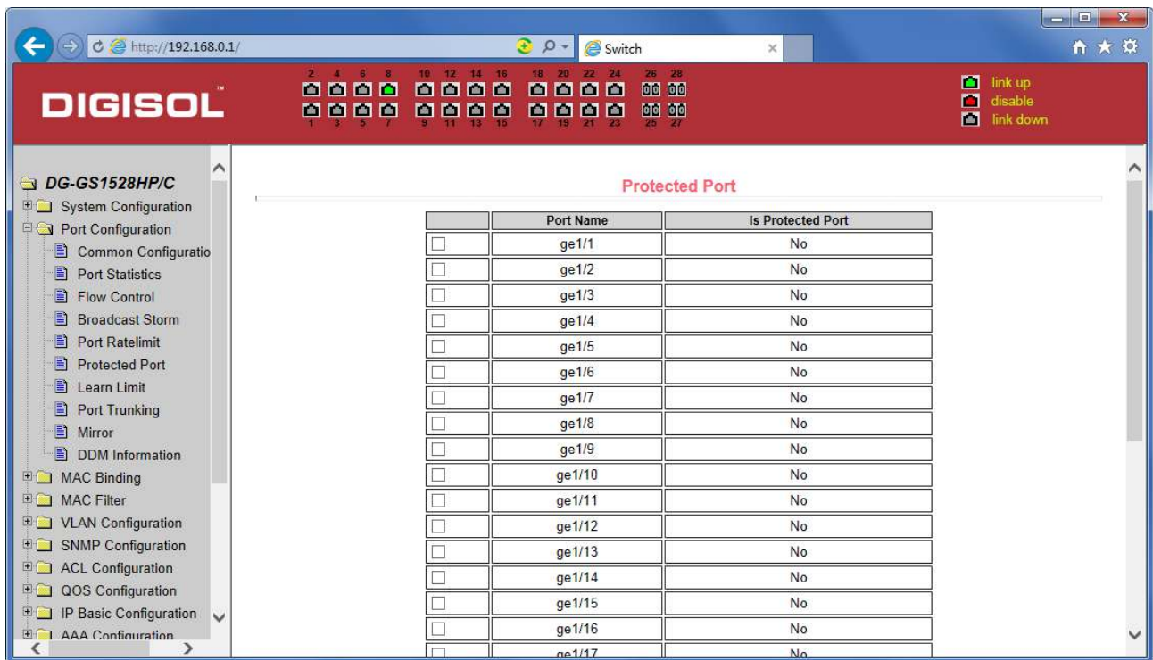
Figure 22 protected port page
