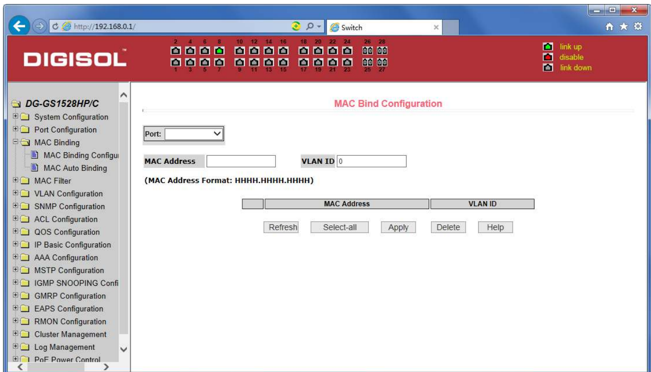
Figure 26 the MAC binding configuration page
