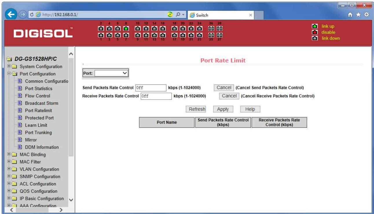
Figure 21 Port speed limit page
