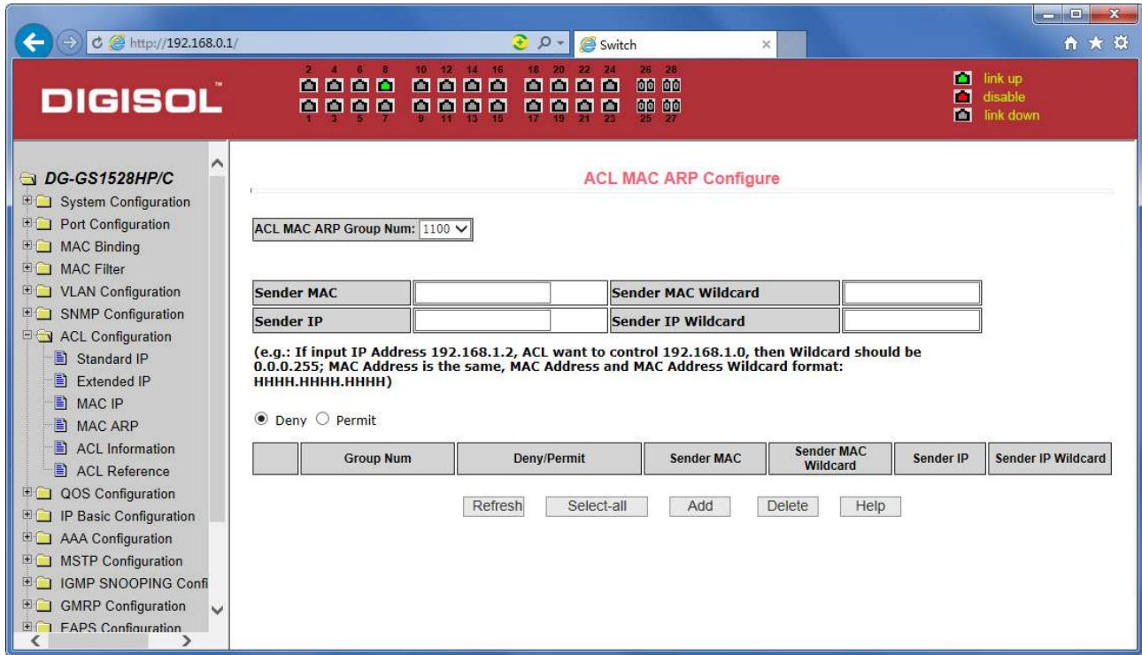
Figure 39 the IP Extended ACL configuration page
