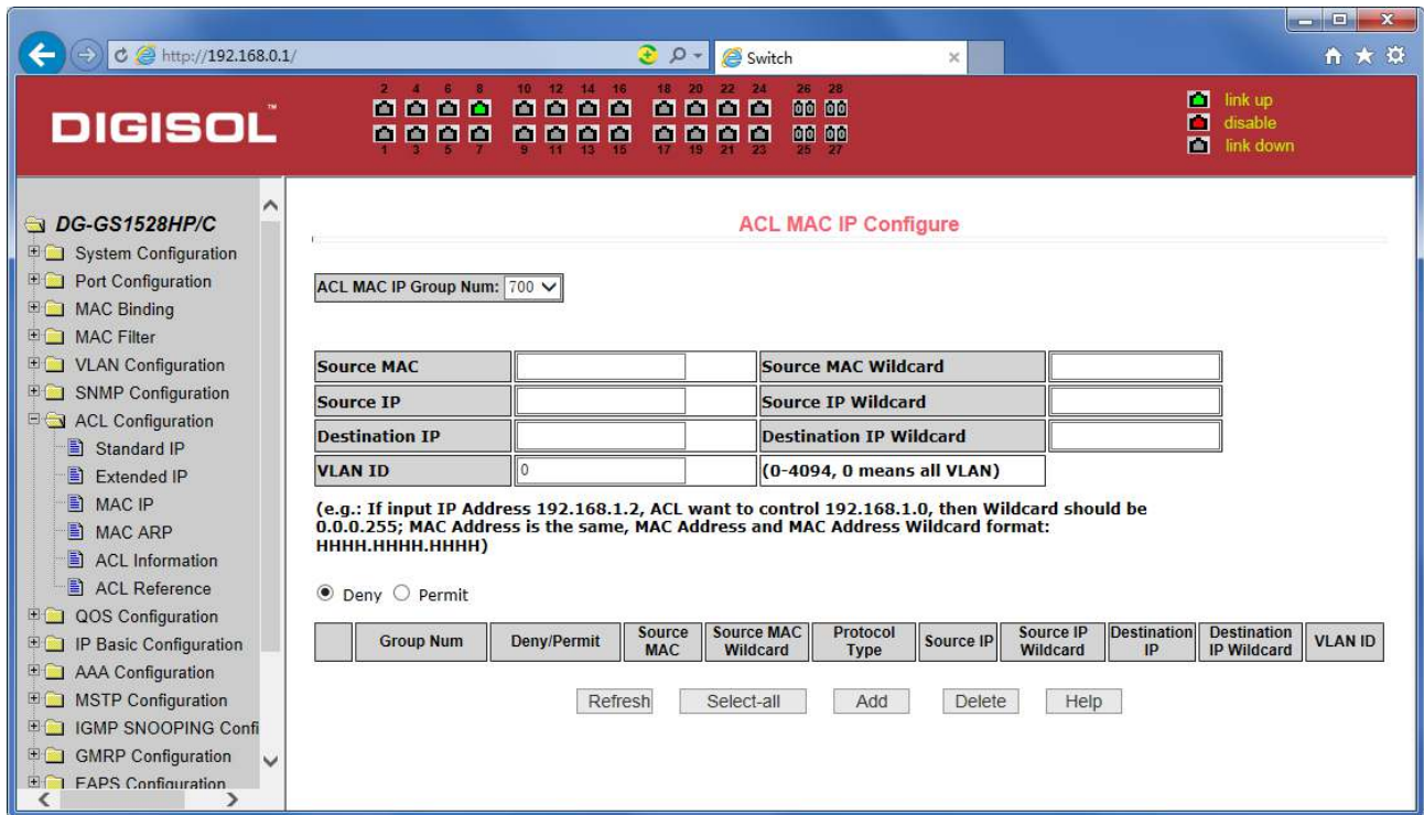
Figure 37 the IP Extended ACL configuration page
