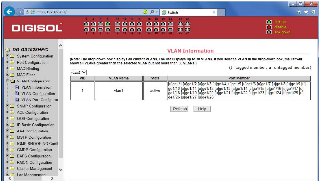
Figure 30 VLAN information page
