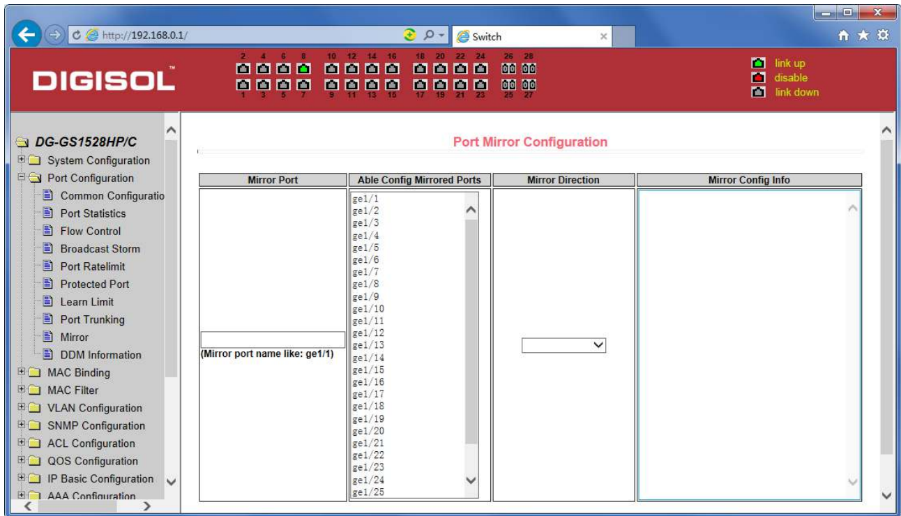
Figure25 Port mirroring configuration page
