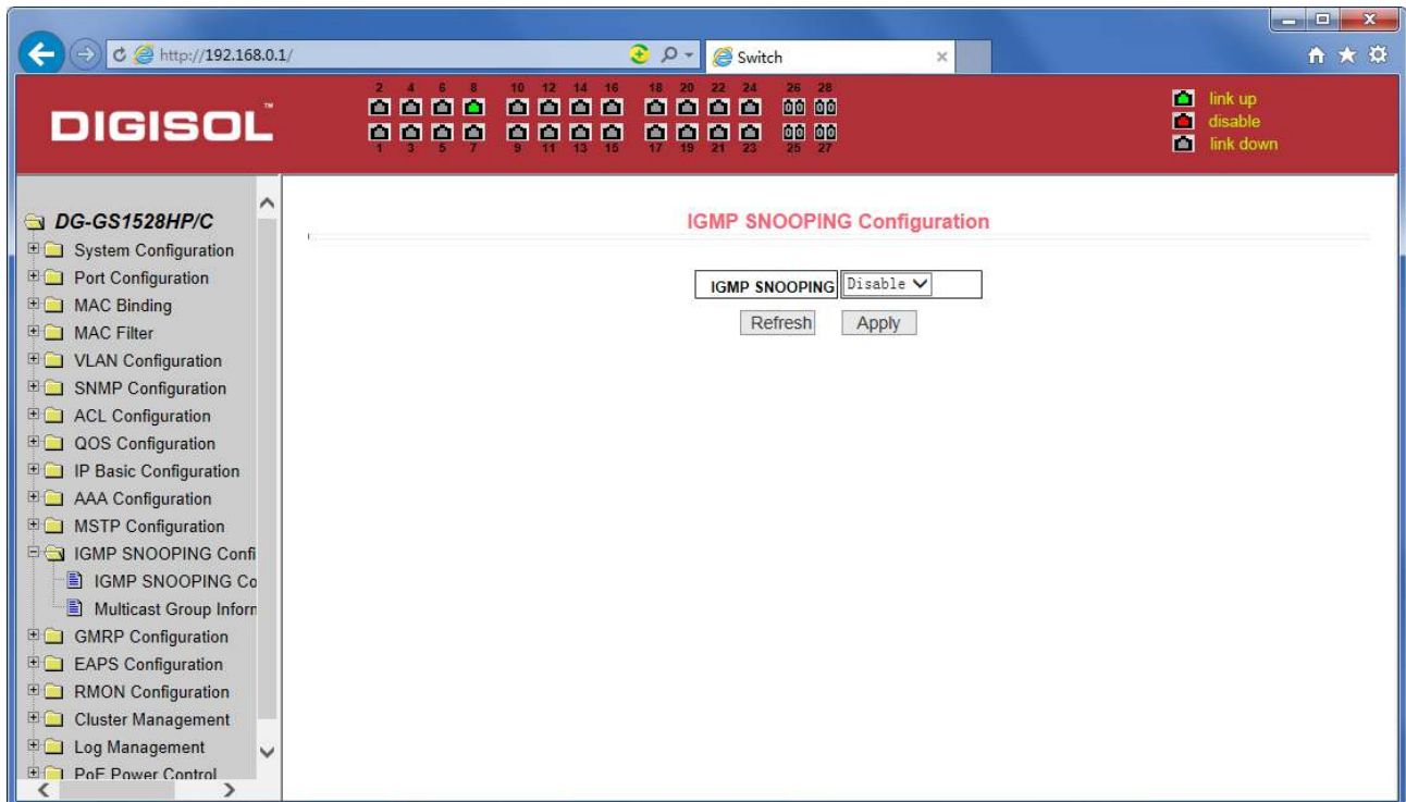
Figure 53 IGMP SNOOPING configuration page
