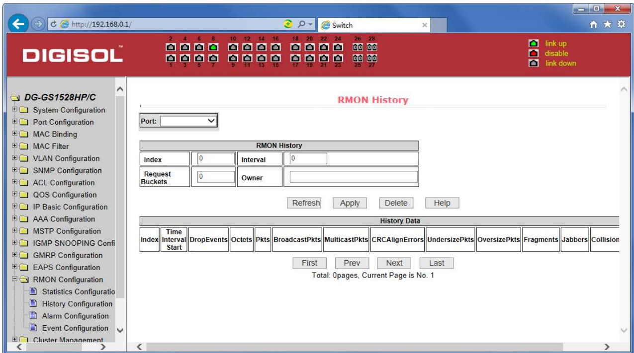
Figure62 RMON history group configuration page
