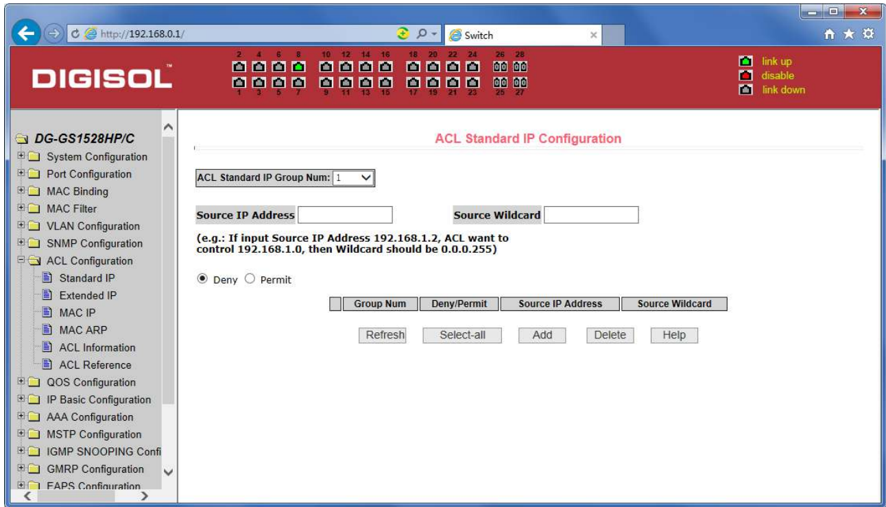
Figure 35 the IP standard ACL configuration page
