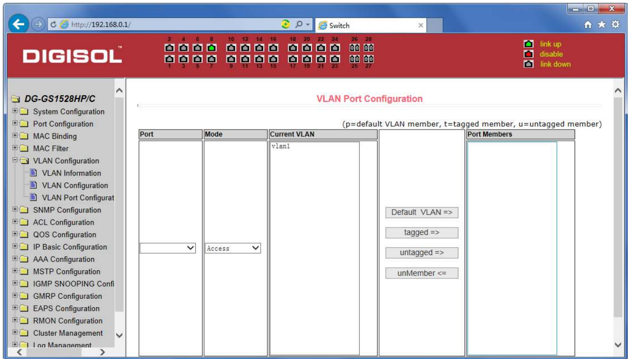
Figure 32 The VLAN port configuration page
