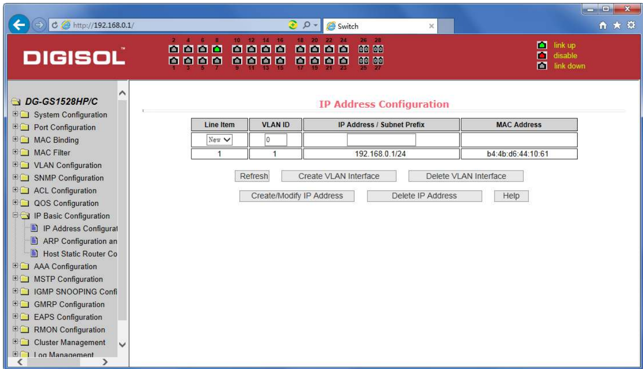
Figure 43 VLAN interface configuration page
