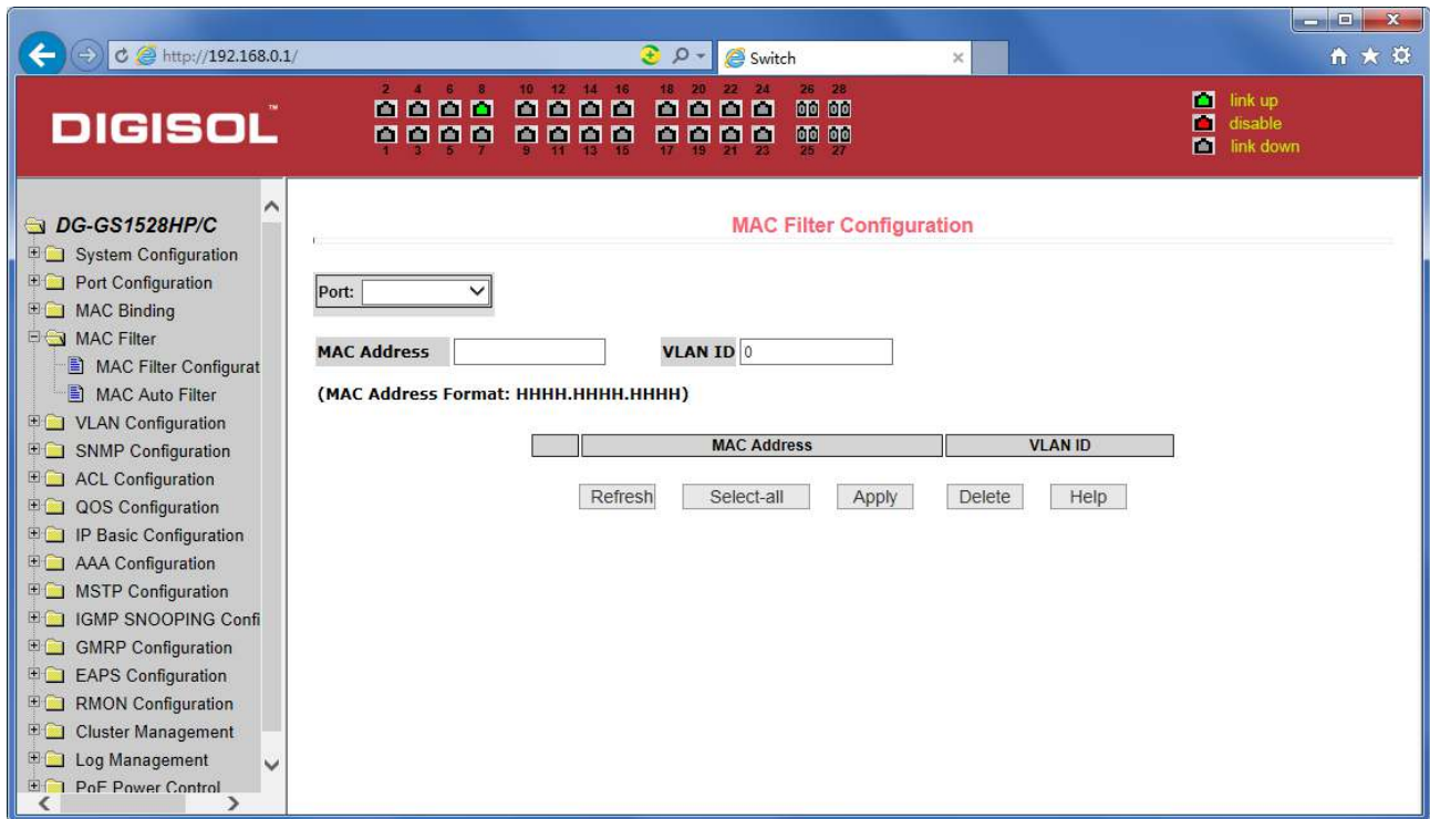
Figure 28 the MAC filtering configuration page
