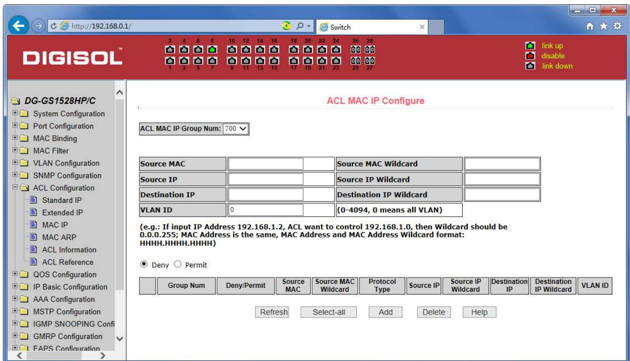
Figure 38 the IP Extended ACL configuration page
