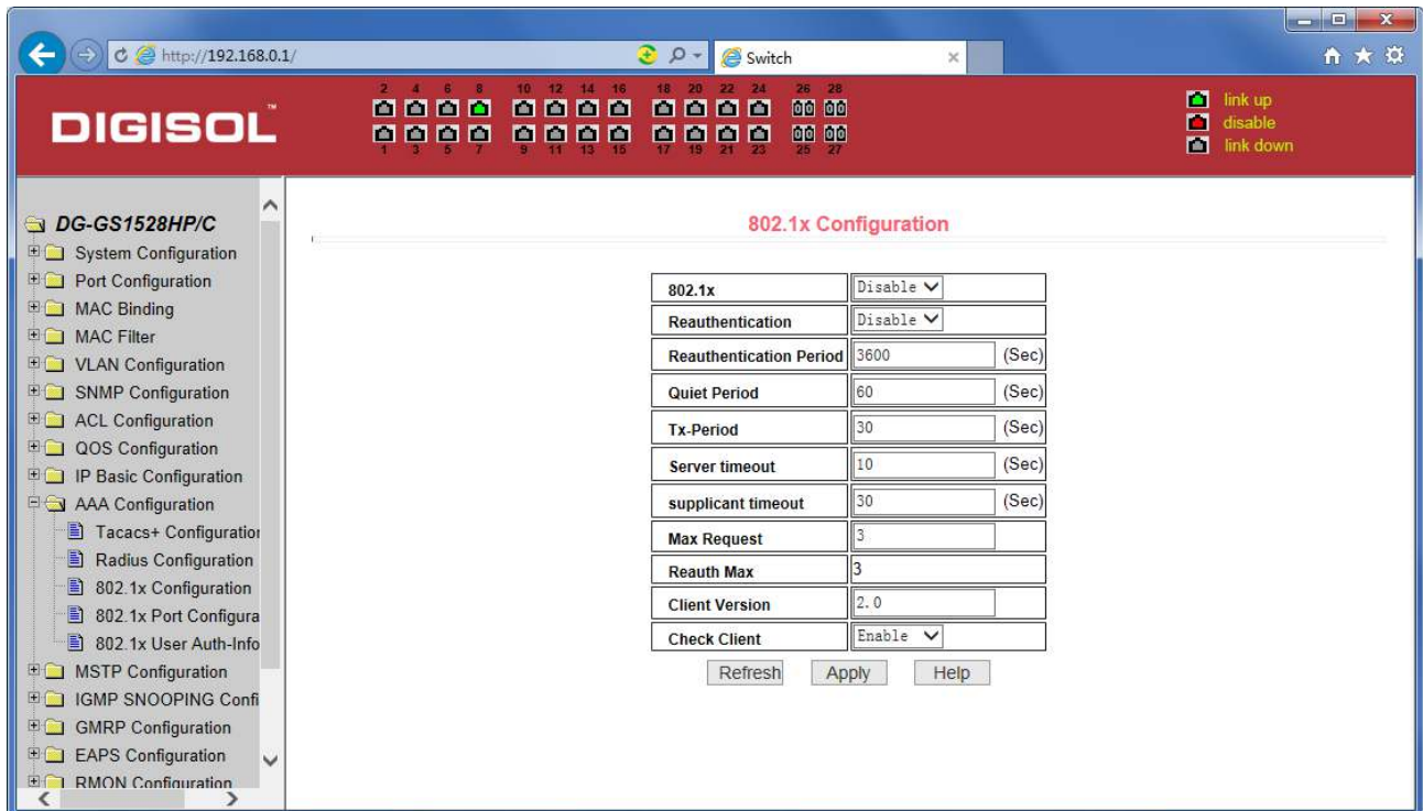
Figure 47 the 802.1x configuration page
