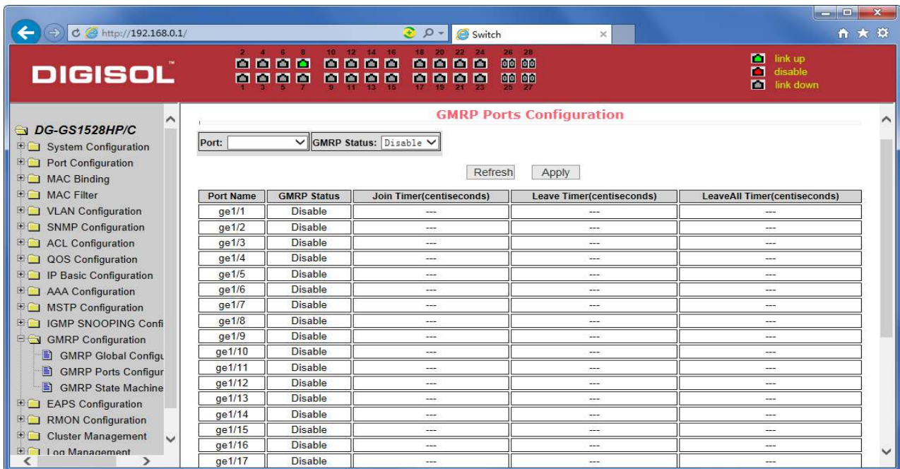
Figure 56 GMRP Port Configuration Page
