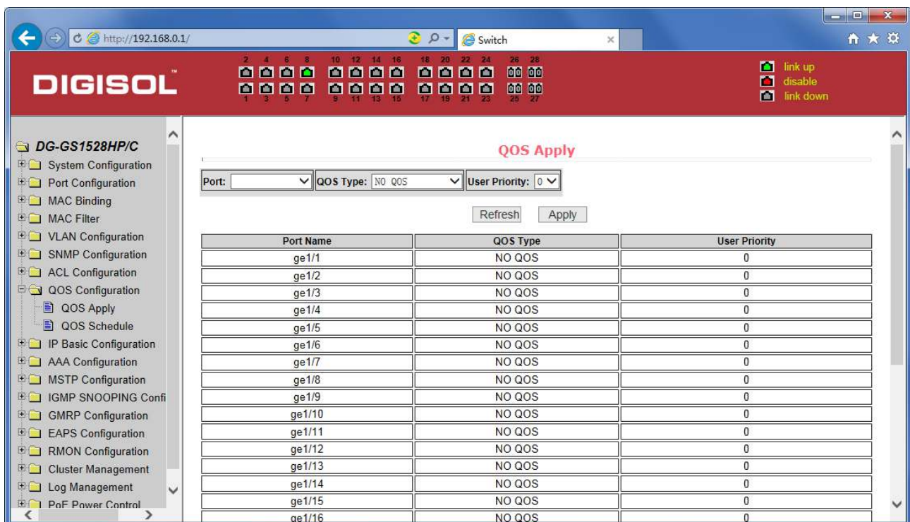
Figure 41 QoS Apply configuration page
