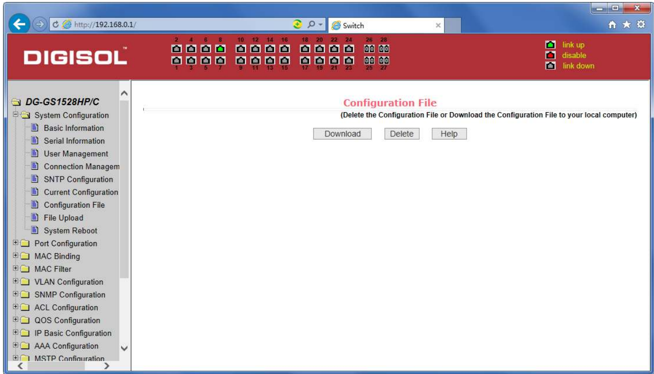
Figure14 Configuration file page
