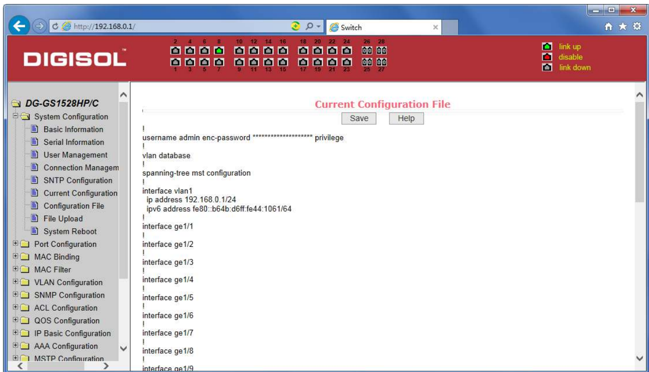
Figure 13 the current configuration page
