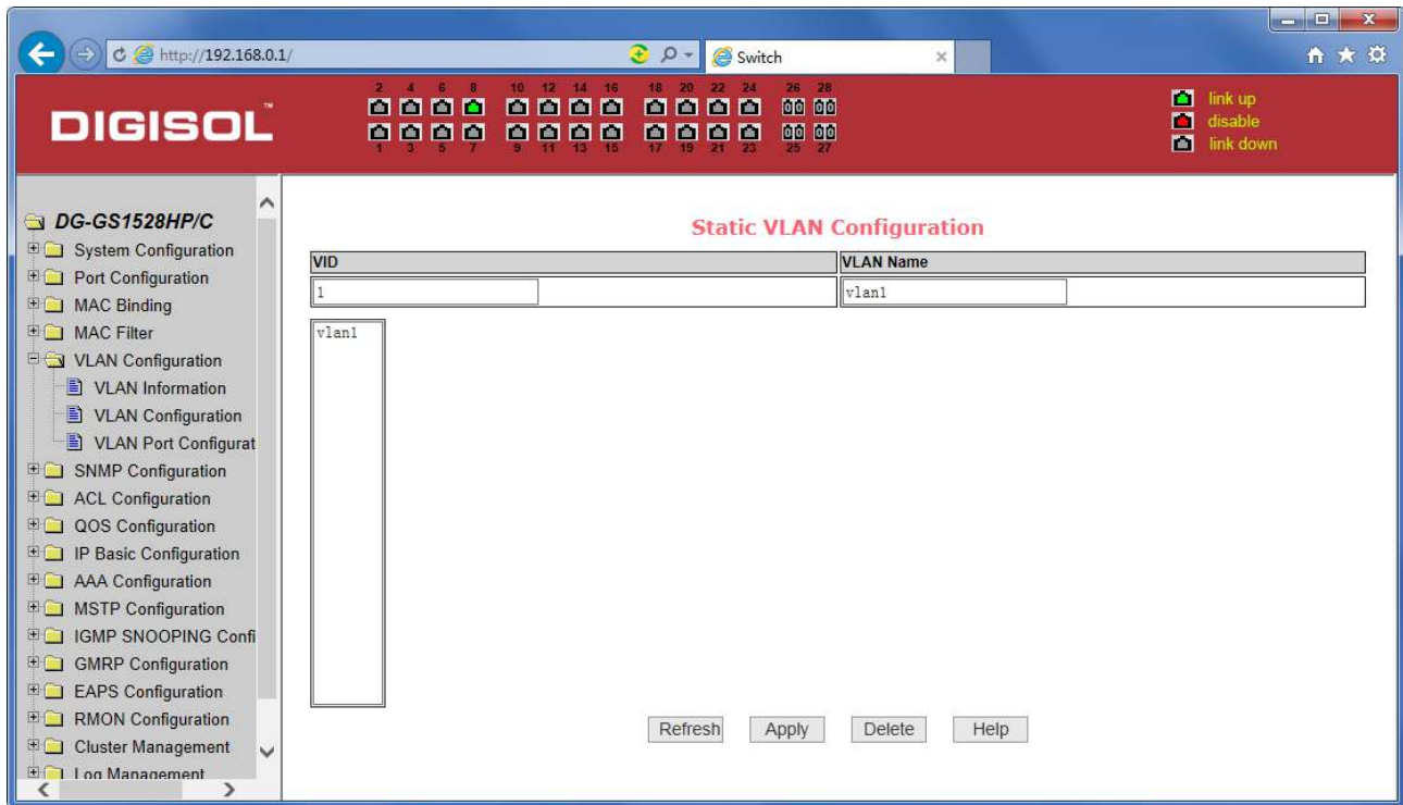
Figure 31 the static VLAN configuration page
