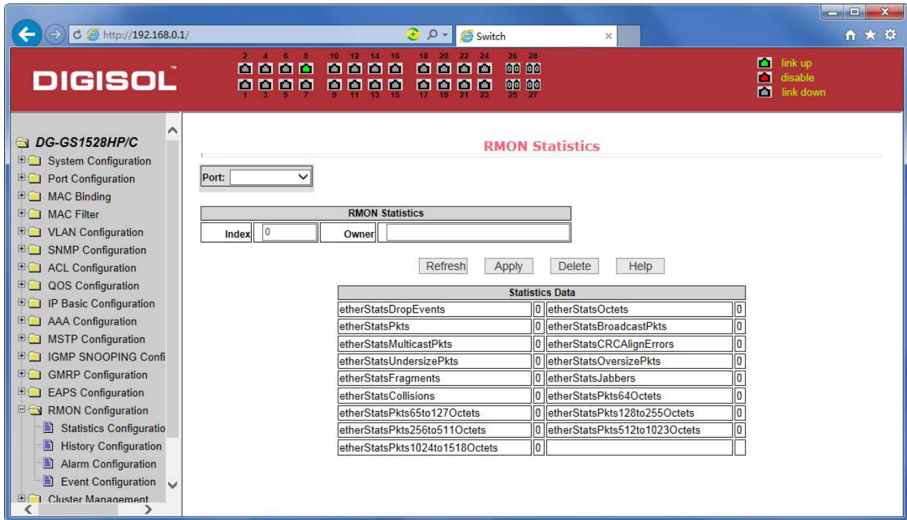
Figure 60 RMON statistics group configuration page
