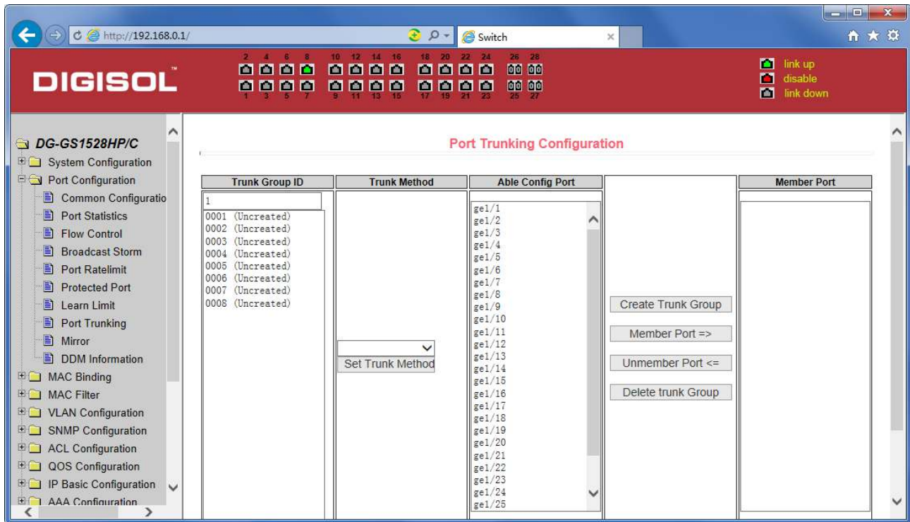
Figure 24 Port Trunking configuration page
