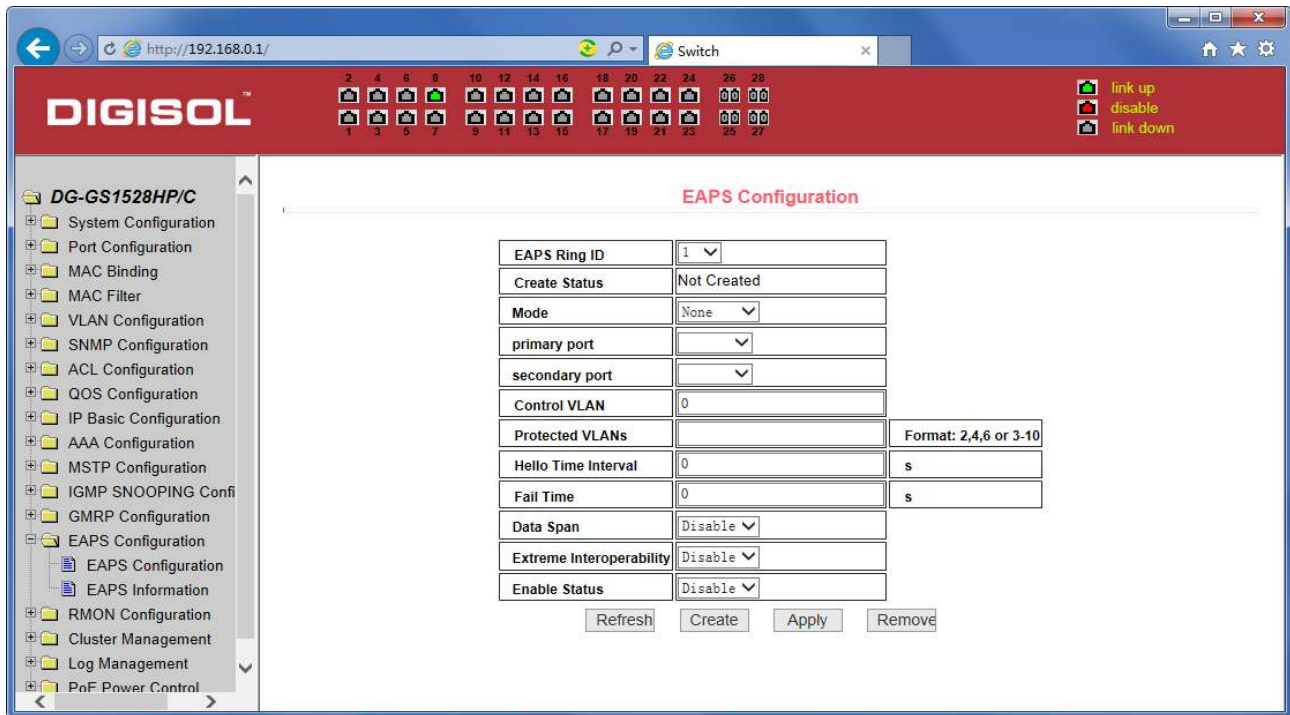
Figure 58 EAPS Configuration Page
