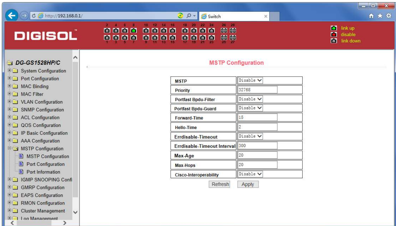
Figure 50 MSTP Global Configuration Page
