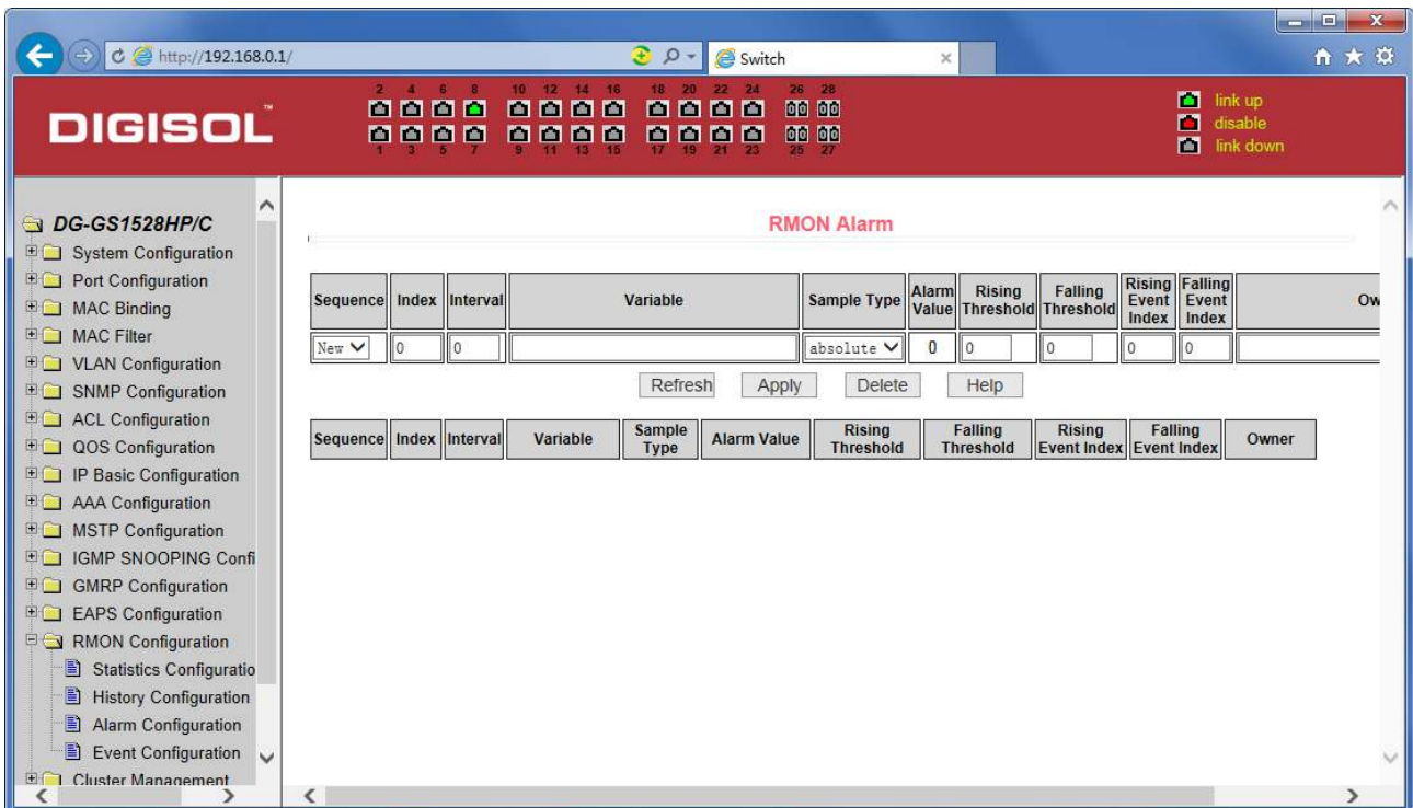
Figure 62 RMON alarm group configuration page
