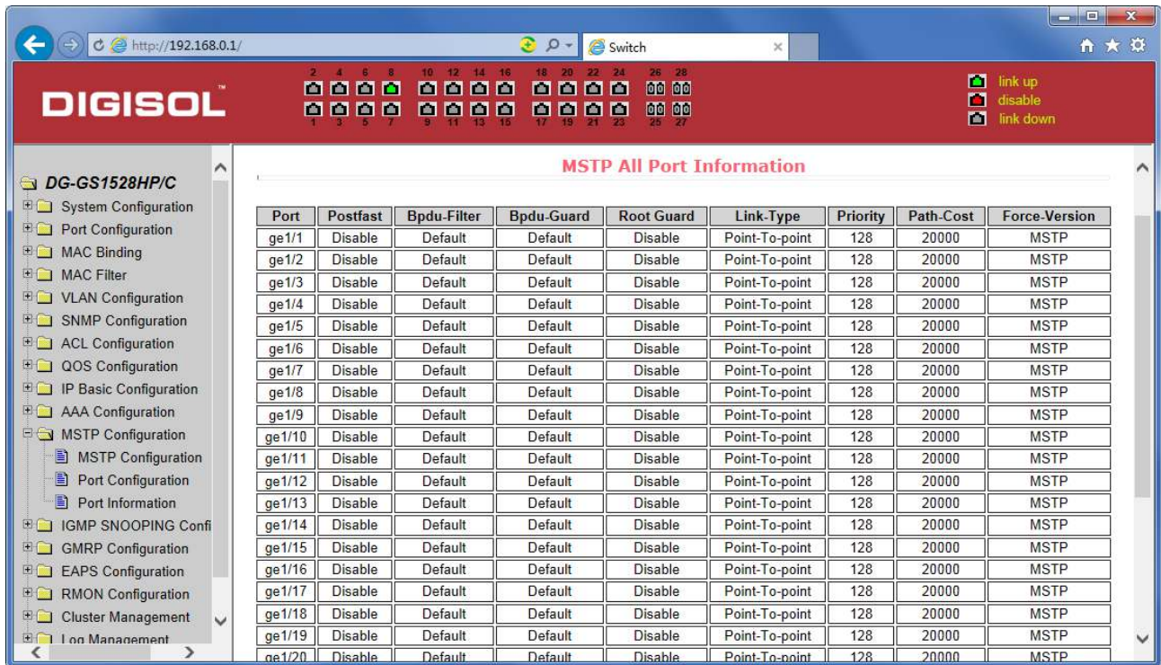
Figure 52 MSTP Configuration Information page
