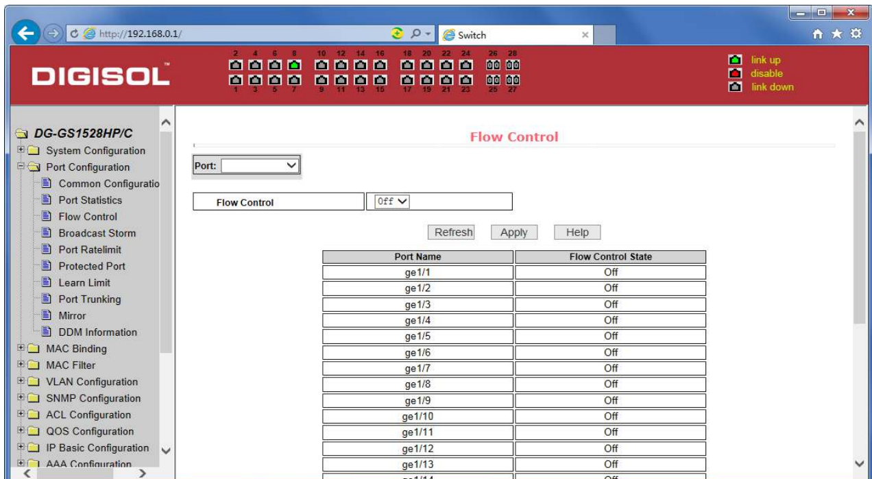
Figure 19 Flow control page
